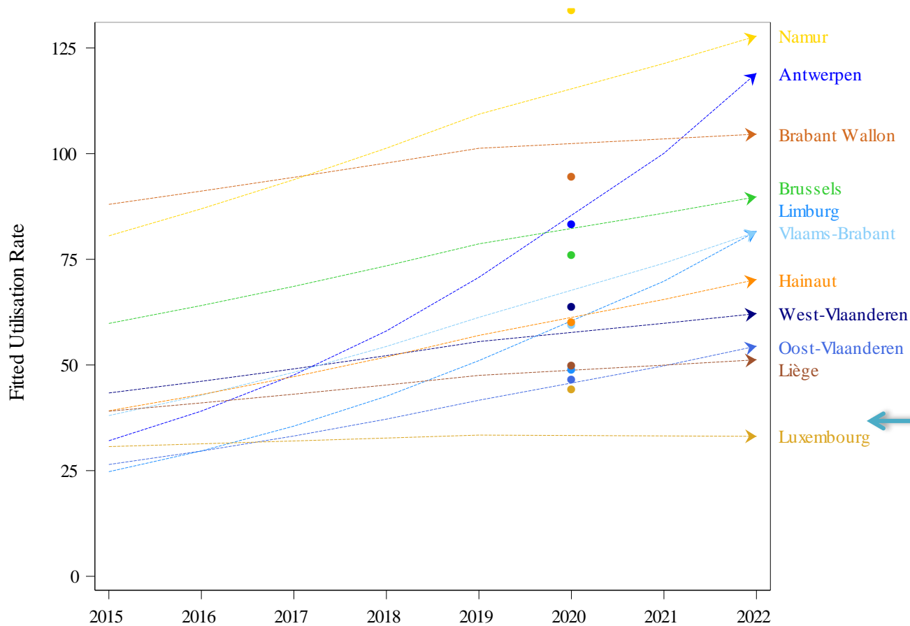
Trend break assessment model by province – Regression lines
